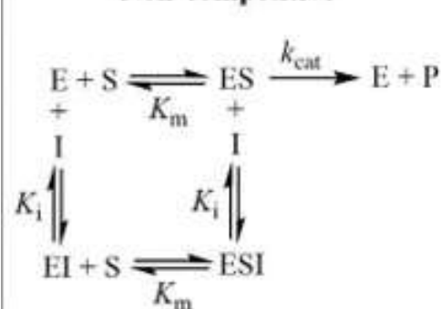
b. Non-competitive inhibitor
