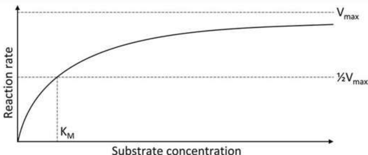
Figure 2. Michaelis–Menten kinetic curve
