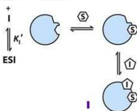
a. Uncompetitive inhibitor
